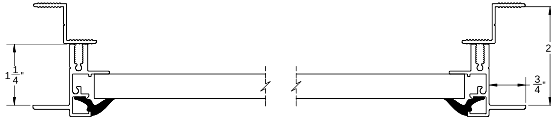
SERIES 1250 SECTION A-A NOT TO SCALE
