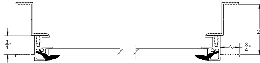
SERIES 1150 SECTION A-A NOT TO SCALE
